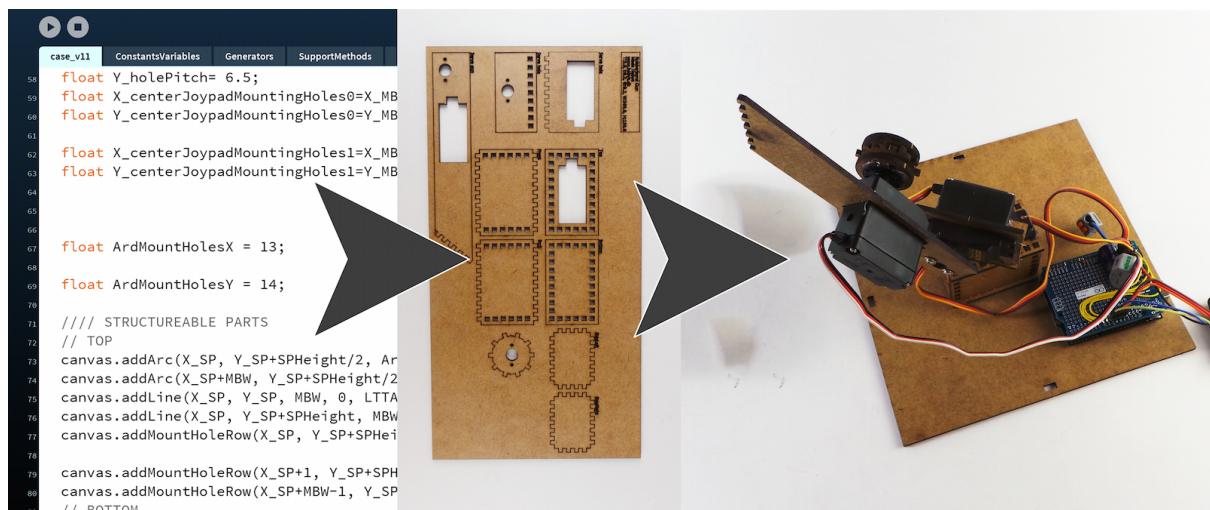
Figure 6: The toolchain of FabMaker. Experienced developers write code that generates “lego”-like pieces that can be combined in endless ways.
