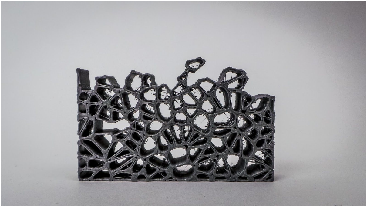
Figure 3: Computationally generated beehive pattern 3D printed in PLA as a prototype for new structures in concrete
